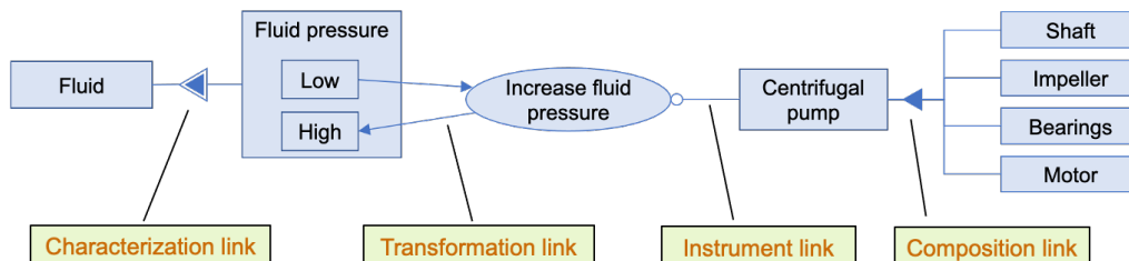
Figure 2. Simplified OPM model of a centrifugal pump.
