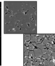
Fig. 3 SEM of the pristine (top) and irradiated (bottom) meta-chert samples showing grain boundary cracking (Maruyama et al. 2022)
