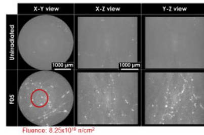
Fig. 1 Void formation on irradiated concrete aggregate
