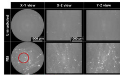
Fluence: 8.25 \times 10^{13} \text{ n/cm}^2 Fig. 2 Void formation on irradiated concrete aggregate
