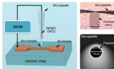
Fig. 2 Scanning electrochemical examination setup (SECM: scanning electrochemical cell microscopy)
