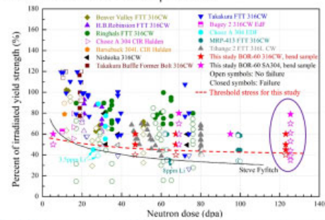
Fig. 3 Minimum stress for IASCC crack initiation in austenitic stainless steels in a PWR primary water environment
