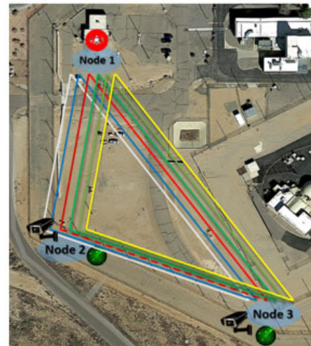
Example of CARBON Wireless nodes using multiple diverse underlay networks to transmit the same data streams
