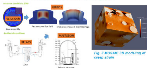
Fig. 2 Assess CBS performance under LOCA and seismic events
