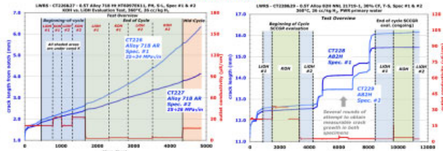
Fig. 3 Similar SCC growth behaviors of Alloy 718 (left) and Alloy 82 (right) in KOH vs. LiOH
