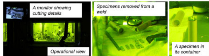
Fig. 2 Weld sample preparation inside hot cell for in-depth characterization
