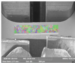
Fig. 1 In-situ tensile testing with SEM and EBSD on EDM machined miniature tensile specimens from harvested baffle former bolt
