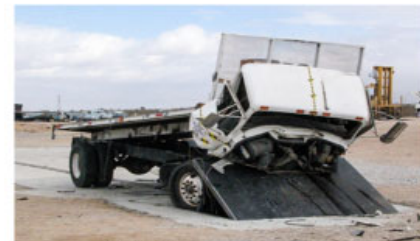
Vehicle Barrier Performance Test
