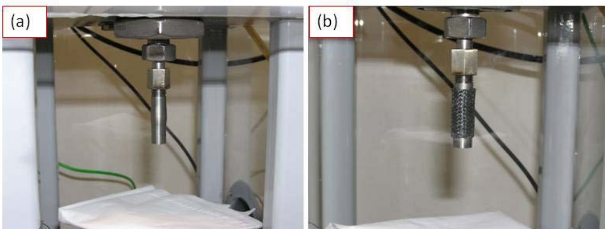
Figure 17. Halden burst-strain test of Zircaloy-4 tubes using a drop-weight apparatus, (a) 9.5% strain in an all-metal rodlet sample at 437 MPa (left) and (b) a Zircaloy-4 tube over-braided with \text{SiC}_f CMC resisted strain up to the test limit of 460 MPa.
