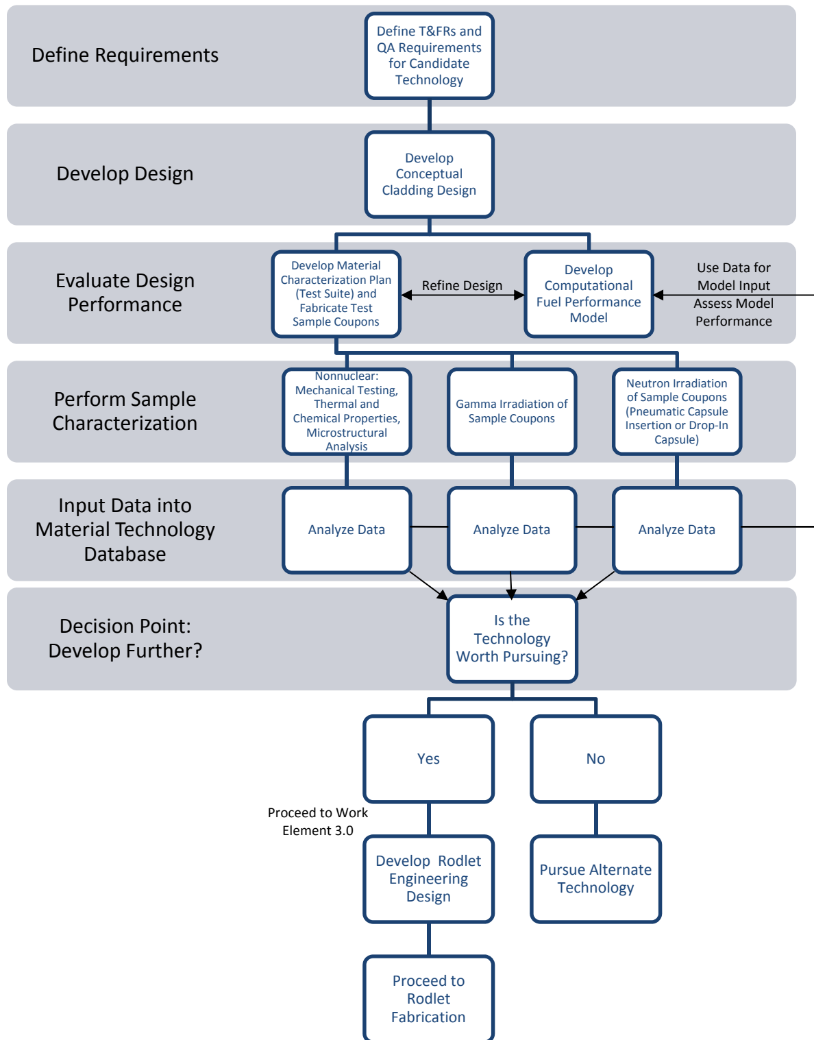
Figure 10. Basic process flow for work element 2.0.
