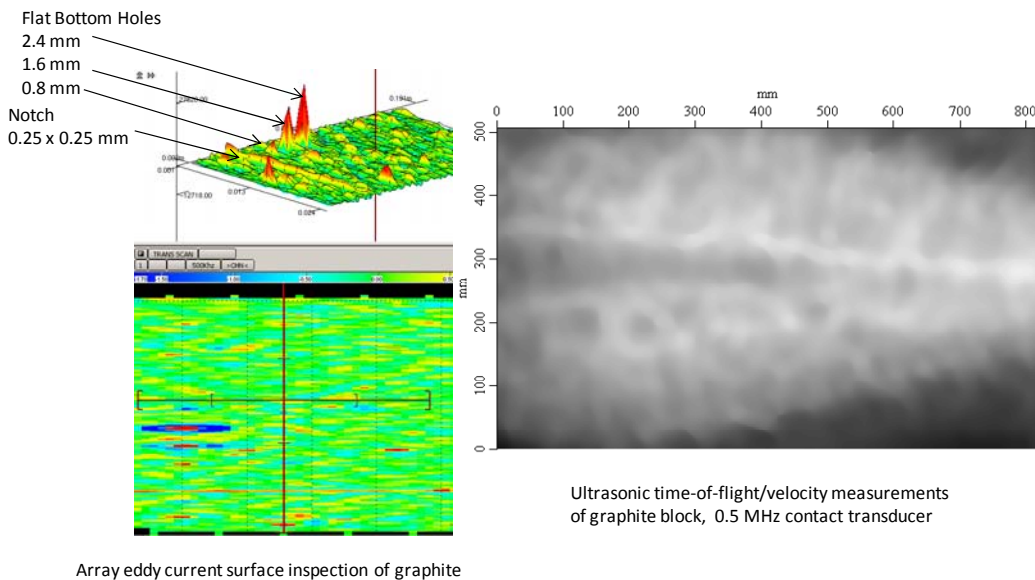
Figure 22. Example non-destructive evaluation techniques.
