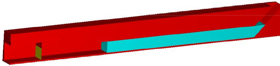
Figure 39. Section of WISD - Inlet angle of 45 degrees and a fluid depth of 1 foot.
