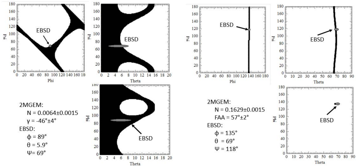
Figure A-3. The possible Euler angles ( \Phi = \phi , \Psi = \psi , \Theta = \theta ) for the orientation of the crystallites of subregions R2b (left) and R5a (right). See the text for a description of the calculation technique. The gray ellipse indicates the measured Euler angles from EBSD, where the extent of the ellipse indicates the estimated error, both stochastic and systematic.
