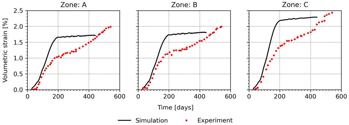
Figure 26: Volumetric strain in zone A, B, and C.
