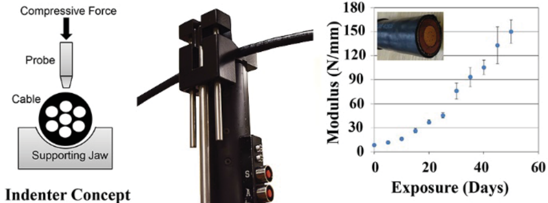
Figure 7.34. Probe, supporting jaw, and cable cross-section ( left ), instrument photo ( center ), and EPR cable modulus vs. exposure time ( right ).
