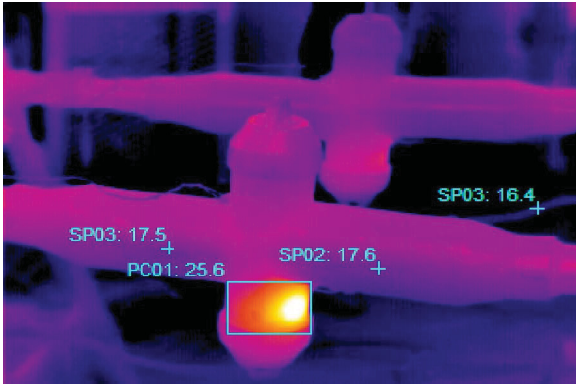
Figure 7.30. IR image – Hot spot in the bulk of insulation of a joint body (pattern 1). Image courtesy of and credited to © Hydro-Québec.
