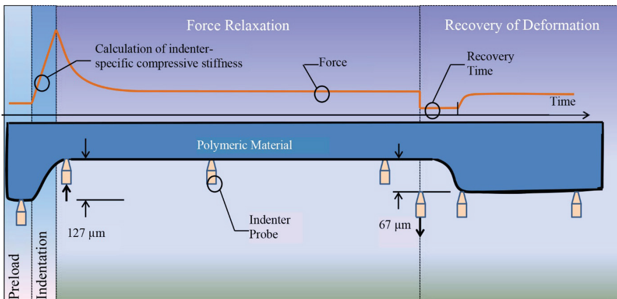
Figure 7.37. A typical test sequence showing the preload, indentation, force relaxation, and deformation recovery phases. The recovery phase is shown following a probe retraction equal to 50% of the initial indentation depth. Figure courtesy of Canadian Nuclear Laboratories.
