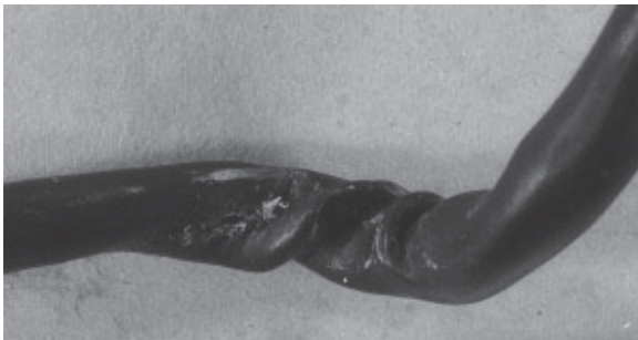
Figure 7.12. Pull-in twist. Photo courtesy of EPRI.
