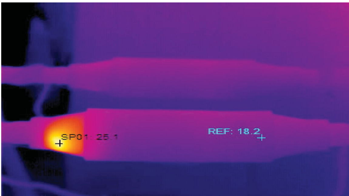
Figure 7.33. IR image – Hot spot in the bulk of insulation located on left side of cable splice. Image courtesy of and credited to © Hydro-Québec.
