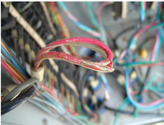
Figure 7.6. Cracks in jacket and insulation. Photo courtesy of EPRI.
