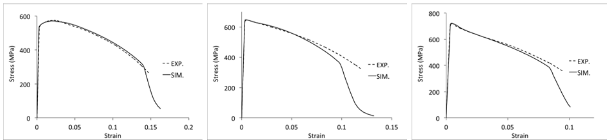
Figure 23: Comparison of engineering stress-strain between FE simulation and experiments for EURO-FER97 irradiated to (a) dpa = 0.06 (b) dpa = 0.6 (c) dpa = 1.5.
