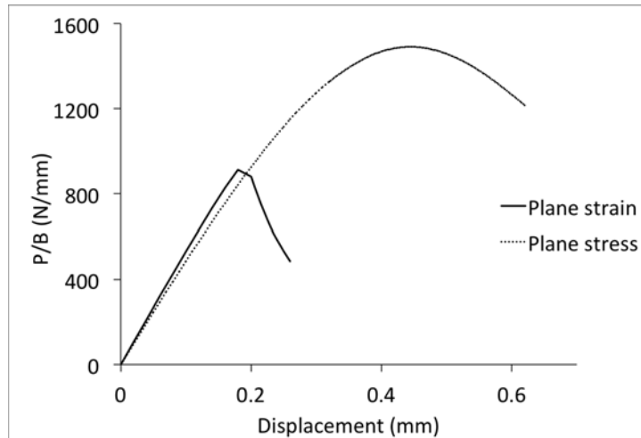
Figure 14: The load-displacement evolution under plane stress and strain conditions obtained from unified CZM based FEM simulations. The cohesive parameters corresponds to T=-100^{\circ}\text{C} and P_f = 5\% .
