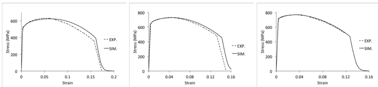
Figure 20: Comparison of engineering stress-strain between FE simulation and experiments for T91 irradiated to (a) \text{dpa} = 0.06 (b) \text{dpa} = 0.6 (c) \text{dpa} = 1.5 .
