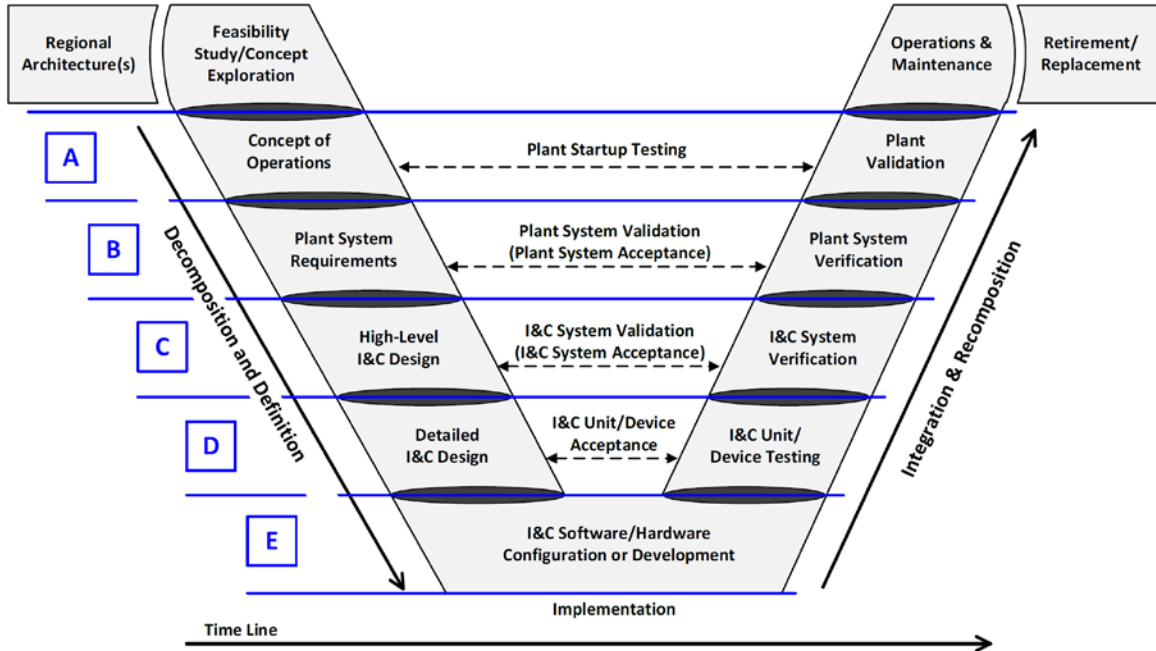
Figure 4 – Systems Engineering Vee Model from the EPRI Digital Engineering Guide.
