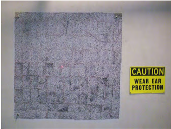
Figure 3. Speckled pattern applied to the upper containment location.
