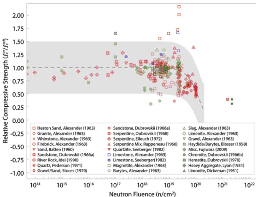
Relative compressive strength of concrete and mortar specimens versus neutron fluence. The neutron spectrum and specimen temperature vary between experiments. Siliceous concrete is depicted with red symbols, calcareous with blue, and miscellaneous concretes with green. Filled symbols indicate experiments conducted above 100°C; open symbols indicate experiments conducted below 100°C.
