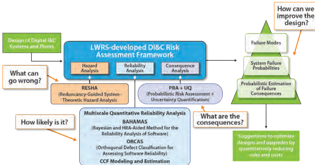
Figure 36. Modularized Structure of Digital I&C System Risk Assessment Framework.
