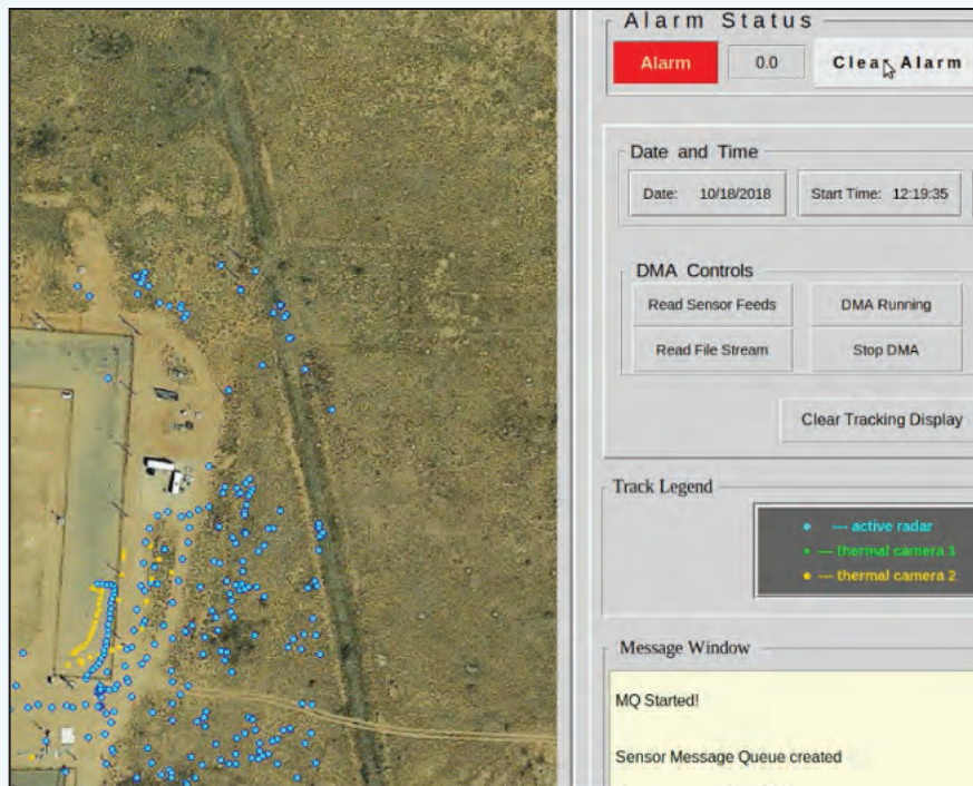
Figure 28. Active Radar (blue) and Thermal Camera (yellow) fused through DMA showing both Nuisance data and Adversary track data.
