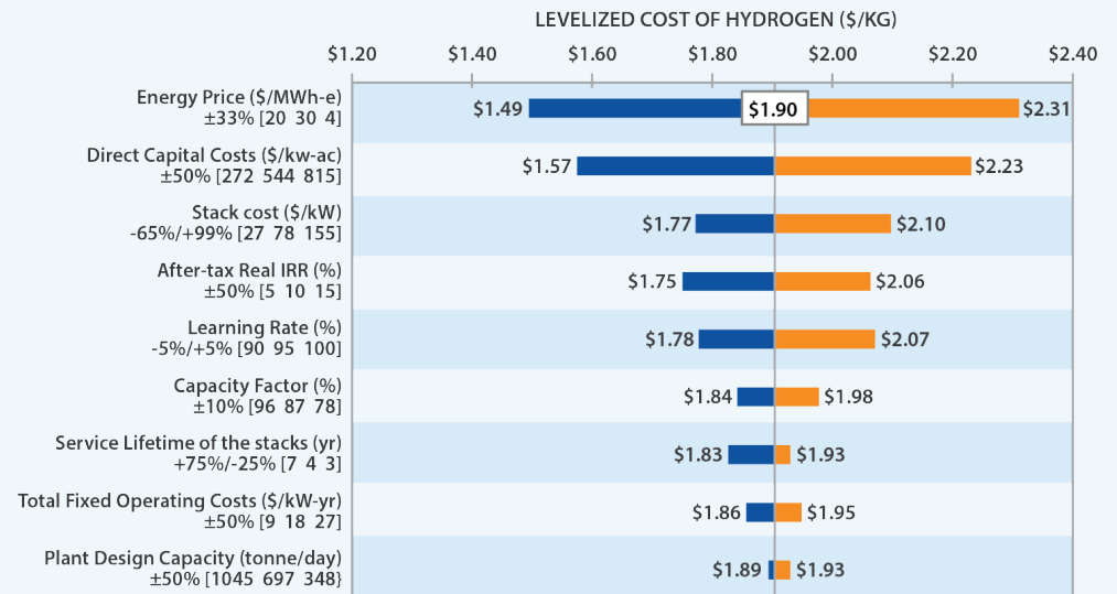
Figure 6. Sensitivity of Levelized Cost of Hydrogen to Price of Electricity, Technology Maturity, Performance Parameters, and Plant Scale.
