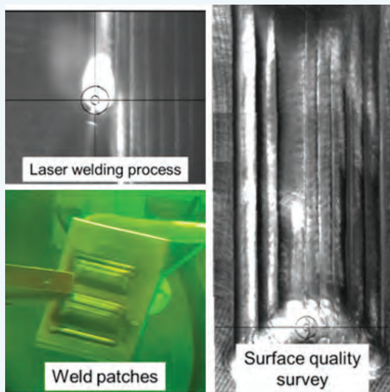
Figure 32. Laser repair welding of irradiated nickel Alloy 182.
