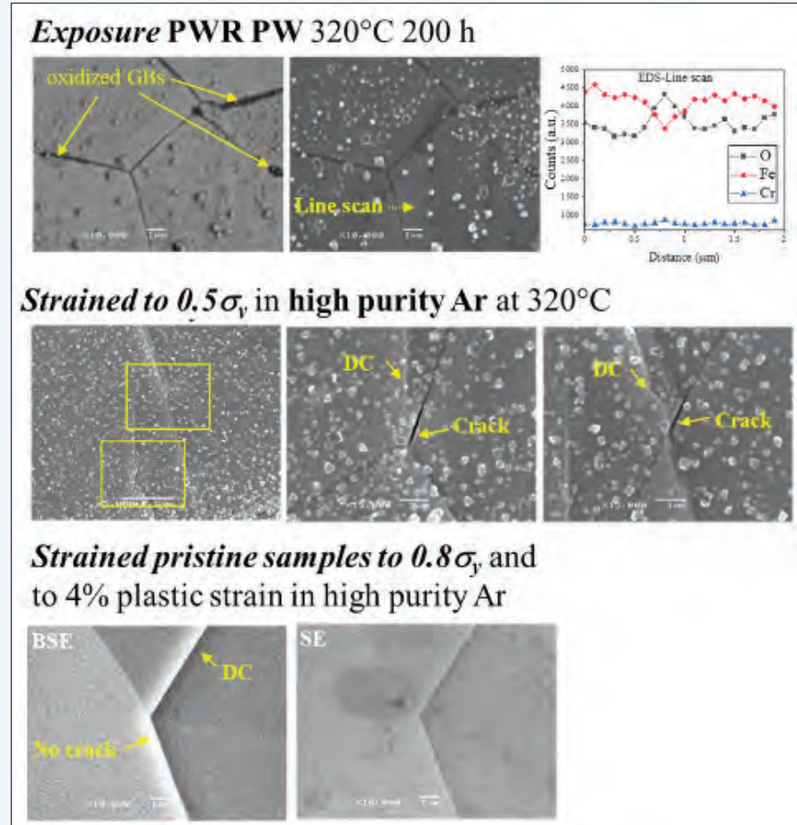
Figure 30. Separation of GB oxidation from intergranular cracking of 304 stainless steel irradiated to 69 dpa in BOR-60 reactor at 320°C. EDS: Energy-dispersive X-ray spectroscopy, DC: dislocation channeling.
