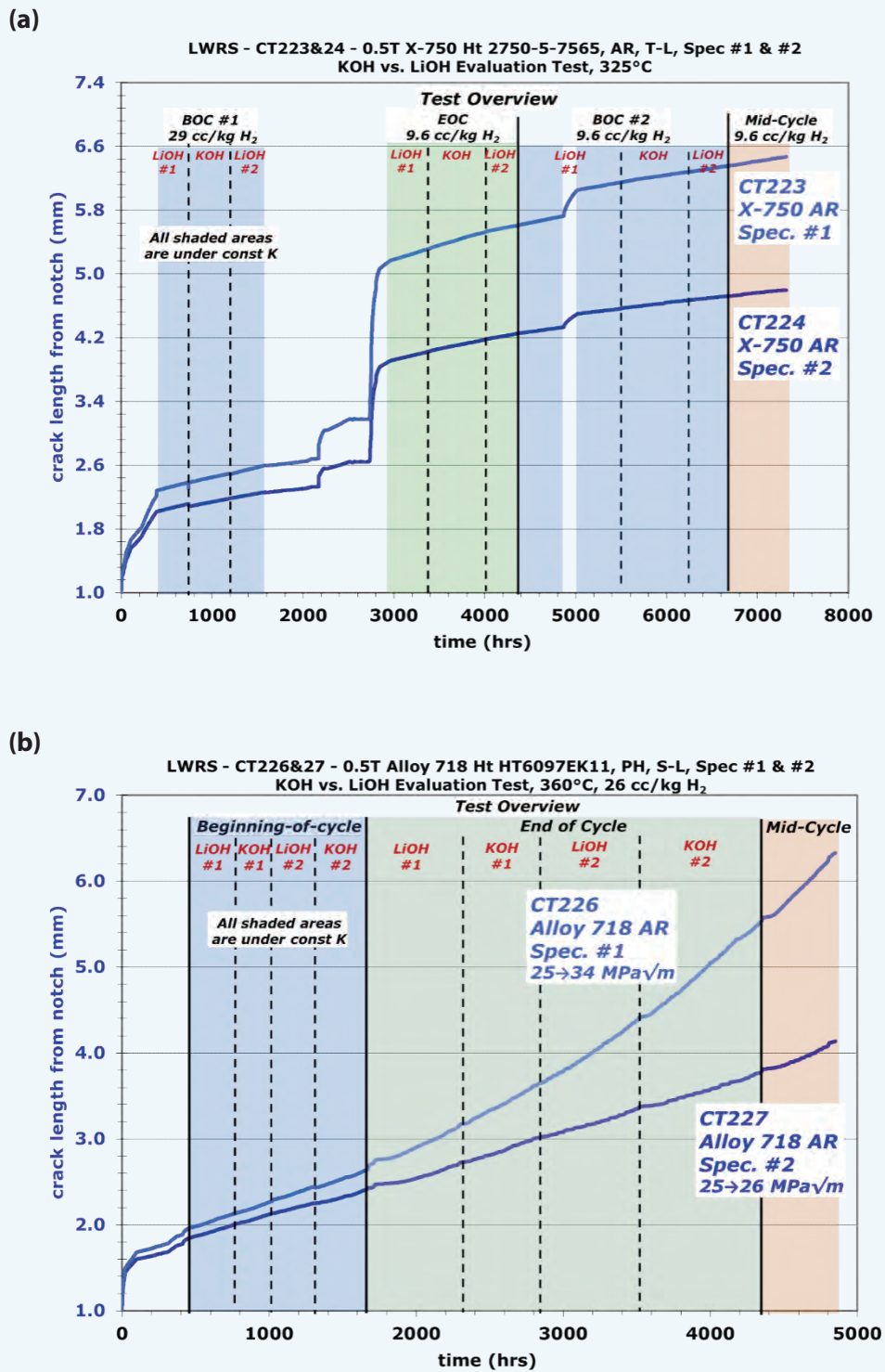
Figure 31. SCC growth behavior of Alloy X-750 in (a) and Alloy 718 in (b) in the beginning-of-cycle, end-of-cycle, and mid-cycle water chemistry with on-the-fly switching between KOH and LiOH.
