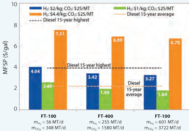
Figure 9. The production cost of Fisher-Tropsch (FT) fuel at different plant scales and H 2 prices. Minimum fuel selling price (MFSP).
