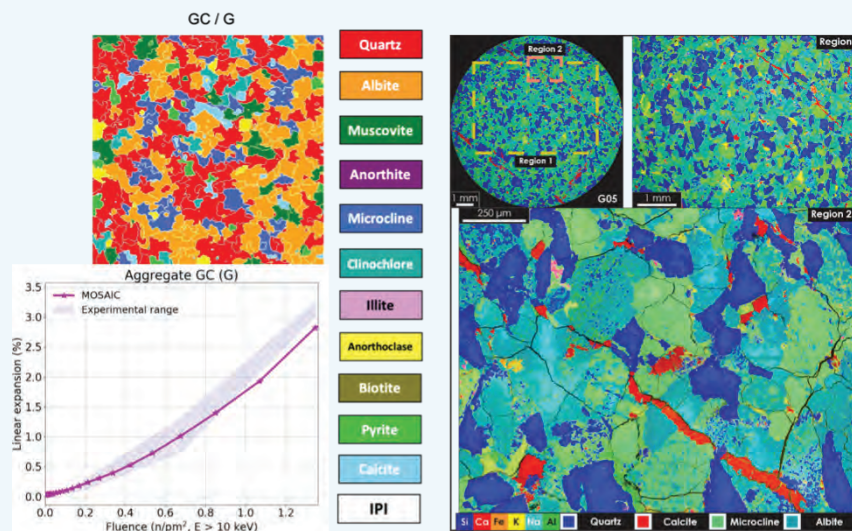
Figure 33. Mineral phase map for a sandstone Japanese aggregate (top left), MOSAIC simulation of aggregate expansion with neutron dose (bottom left), and micro-crack observation through microscopy and spectroscopy showing cracks along grain boundaries and through mineral grains. Note no cracks are observed through quartz grains (dark blue particles).
