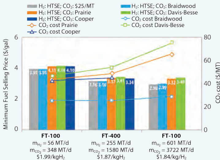
Figure 10. Influence of nuclear power plant location and CO 2 price on the production of FT synfuel.
