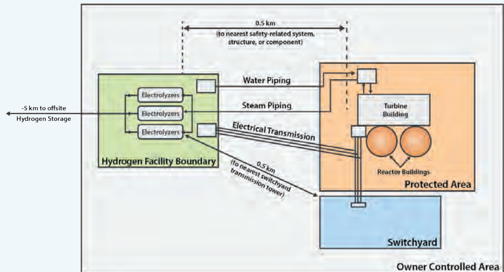
Figure 3. Architecture/Engineering conceptual site layout for a 100 MWe hydrogen facility design.
