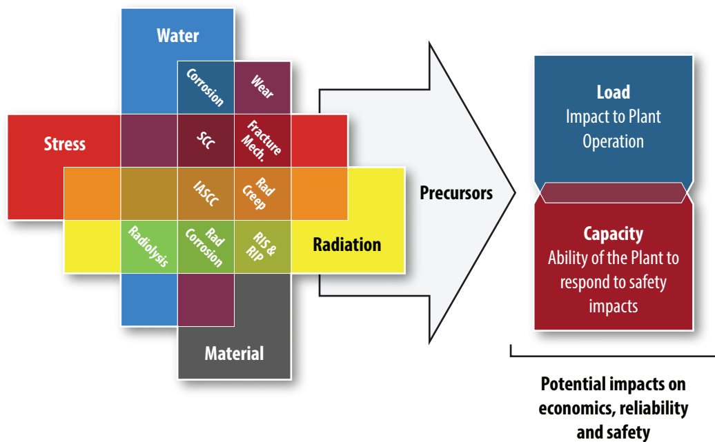
Figure 29. Complexity of interactions between materials, environments, and stresses in a nuclear power plant. SCC: stress corrosion cracking, IASCC: irradiation-assisted stress corrosion cracking, RIS: radiation-induced segregation, RIP: radiation-induced precipitation.
