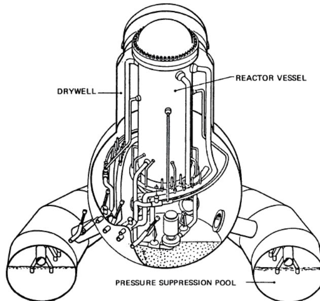
Figure 3-1 View of the BWR Mk.I system
