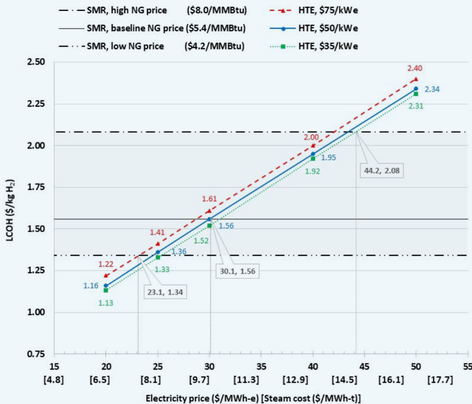
Figure 14. Comparison of hydrogen production costs for electrolysis versus conventional natural gas reforming.
