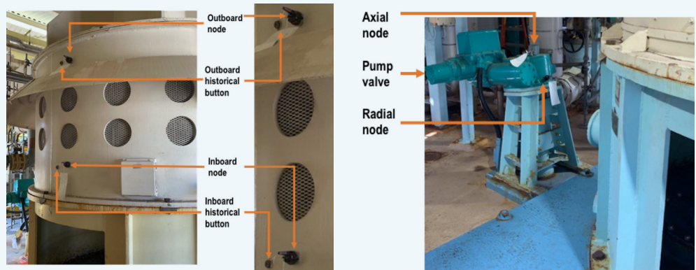
Figure 5. VSN locations for CWP motors (left) and pump valves (right); VSNs are in close proximity to the locations where historical vibration data has been taken for CWP motors.
