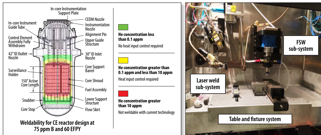
Figure 21. (left) Forecast of helium generation at 75 wppm boron at 60 effective full-power years. Red Zone: >10 appm He (not weldable with current welding processes); Yellow Zone: 0.1 to 10 appm He (weldable with heat-input control during welding repair); Green Zone: <0.1 appm He (no special process control is needed in welding repair). 31 (right) Inside view of the laser and friction-stir weld sub-systems installed in the hot-cell cubicle for testing irradiated materials.
