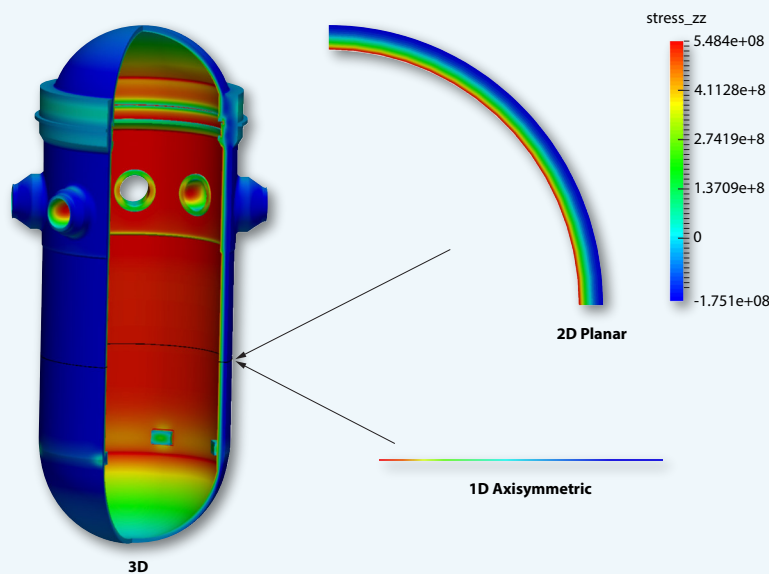
Figure 19. Results of one-dimensional axisymmetric, two-dimensional (2D) planar, and 3D Grizzly models of the global response of an RPV at a point in time during a pressurized thermal shock event.
