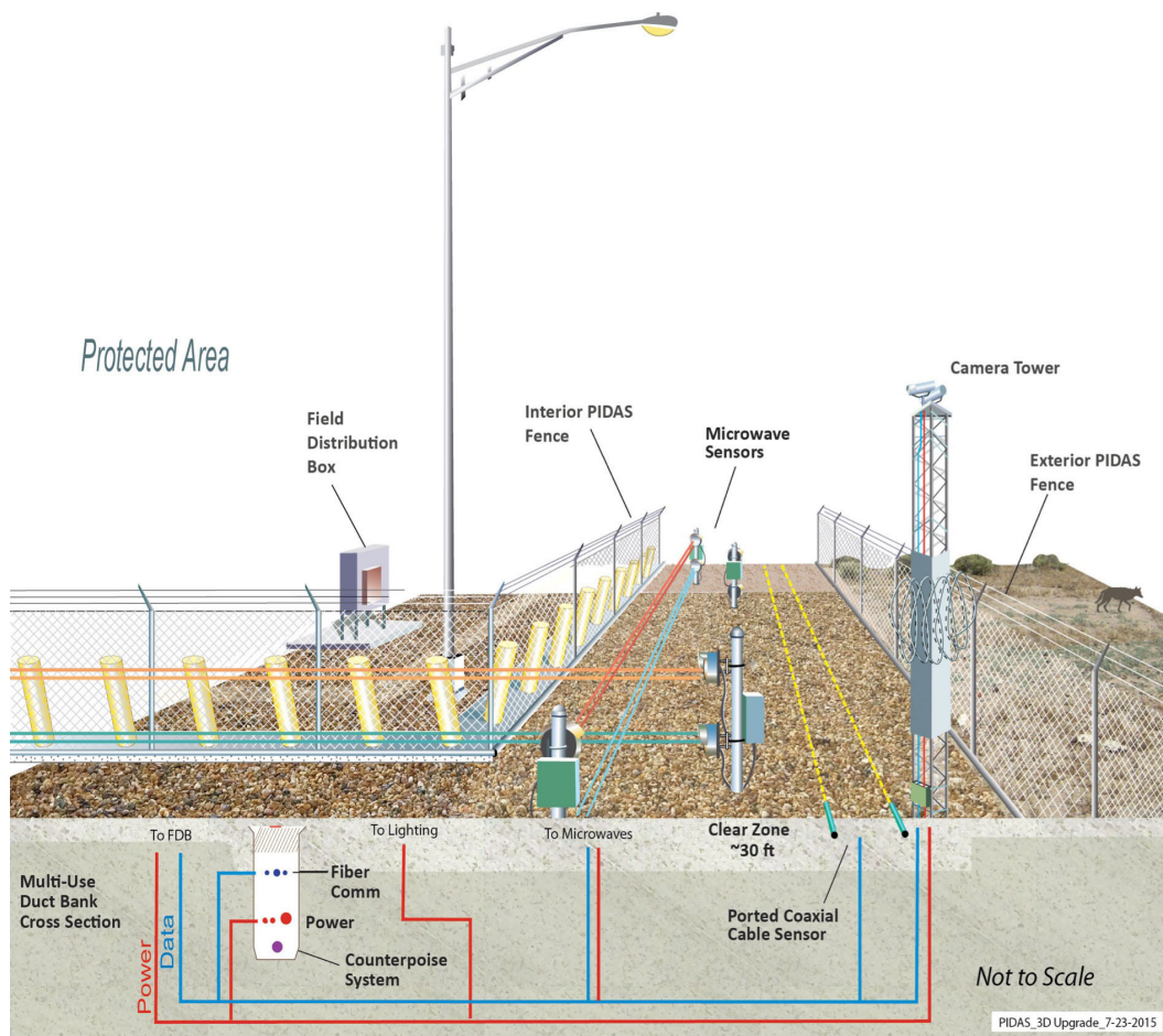
Figure 10. Example of current PIDAS technologies at a nuclear power plant site for adversary detection and assessment entering the protected area.
