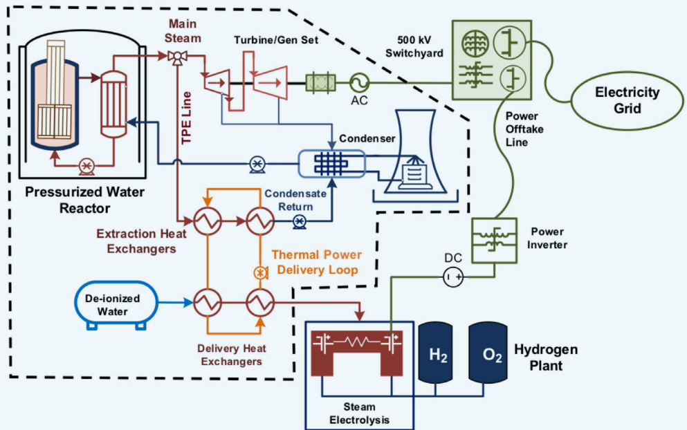
Figure 15. Boundary limits of the Thermal Power Dispatch GPWR Simulator (dashed line).
