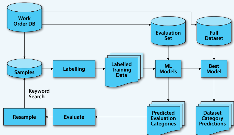
Figure 6. Work order classifier natural language process workflow.
