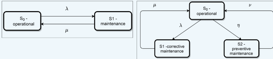
Figure 7. Two-state (left) and three-state (right) Markov models. Here \lambda is the failure rate; \mu is the corrective maintenance rate; \eta is the preventive maintenance scheduling rate; and \nu is the preventive maintenance rate.
