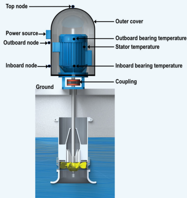
Figure 4. Mounting location of the VSN on the CWP motor.
