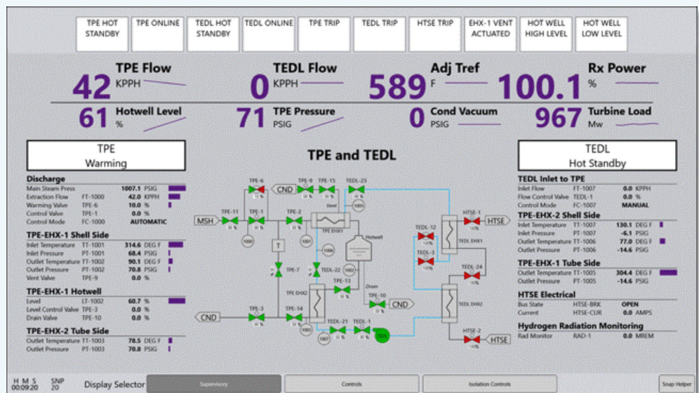
Figure 16. Human system interface design used for conducting human in the loop studies of operating a hybrid energy system integrated in a pressurized water reactor.
