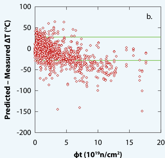
Figure 18. Plot of the difference between the predicted and measured change in Temperature °C vs Fluence.
