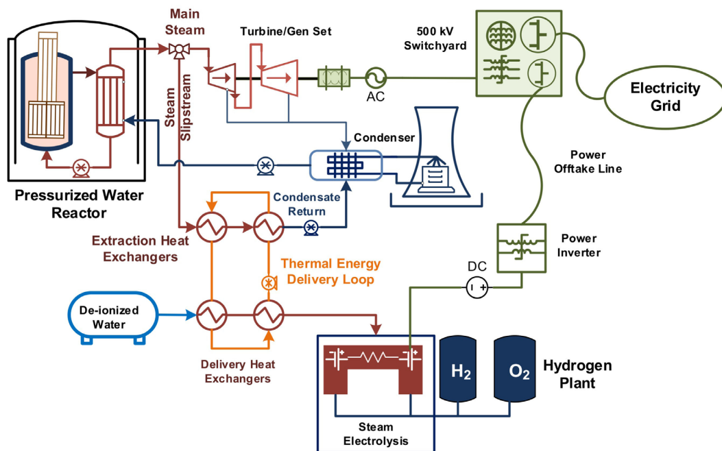
Figure 12. Conceptual design of a hybrid Flexible Plant Operation and Generation plant producing hydrogen and grid electricity.
