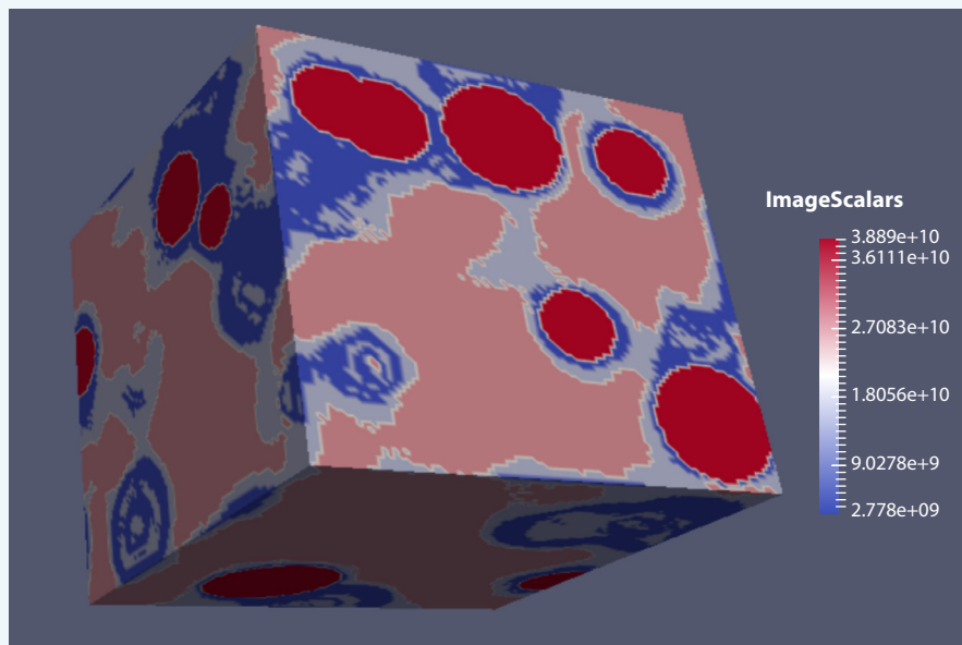
Figure 20. Microstructure and stiffness map showing damaged areas after thermal expansion of the aggregates.
