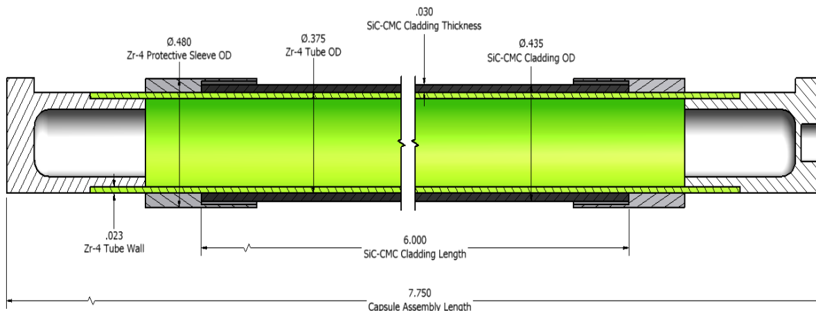
Figure 2. Geometry of the LWRS capsule assembly design for the SiC-CMC hybrid Zr-4 cladding rodlet[3].
