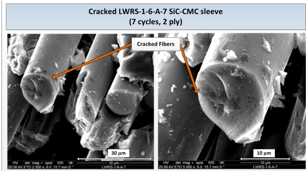
Figure 70. Figure showing SEM images of the fractured fibers of the LWRS-1-6-A-7 SiC-CMC sleeve at crack area 1.
