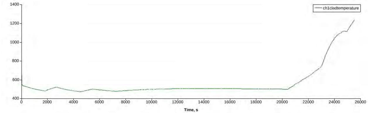
Figure 29. Peak clad temperature for the Scenario II with larger reactor core isolation cooling flow rate .
