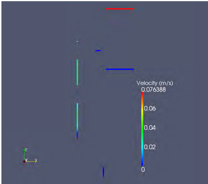
Figure 13. RELAP-7 calculated fluids velocity at the end of simulation for Scenario I.
