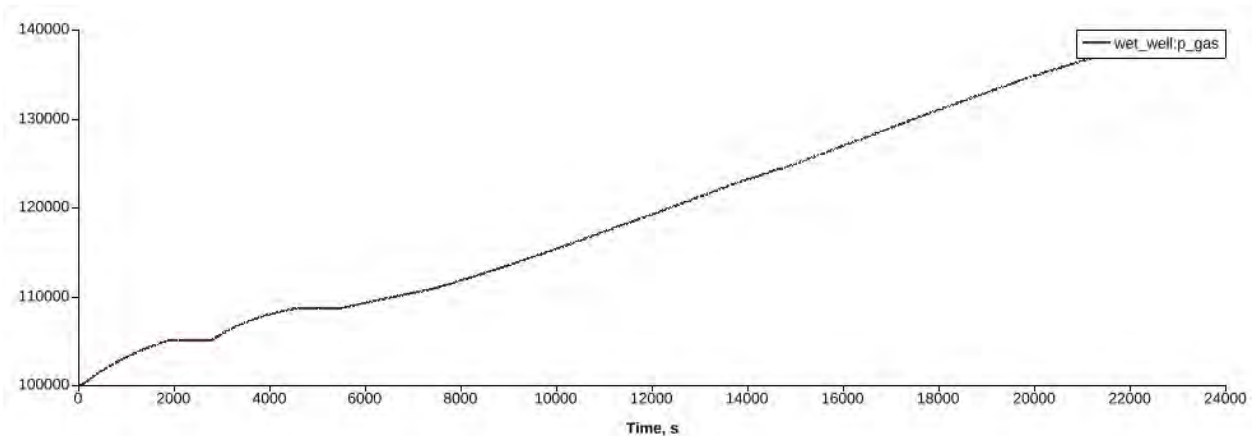
Figure 25. Wet well gas space pressure for the Scenario II base case.
