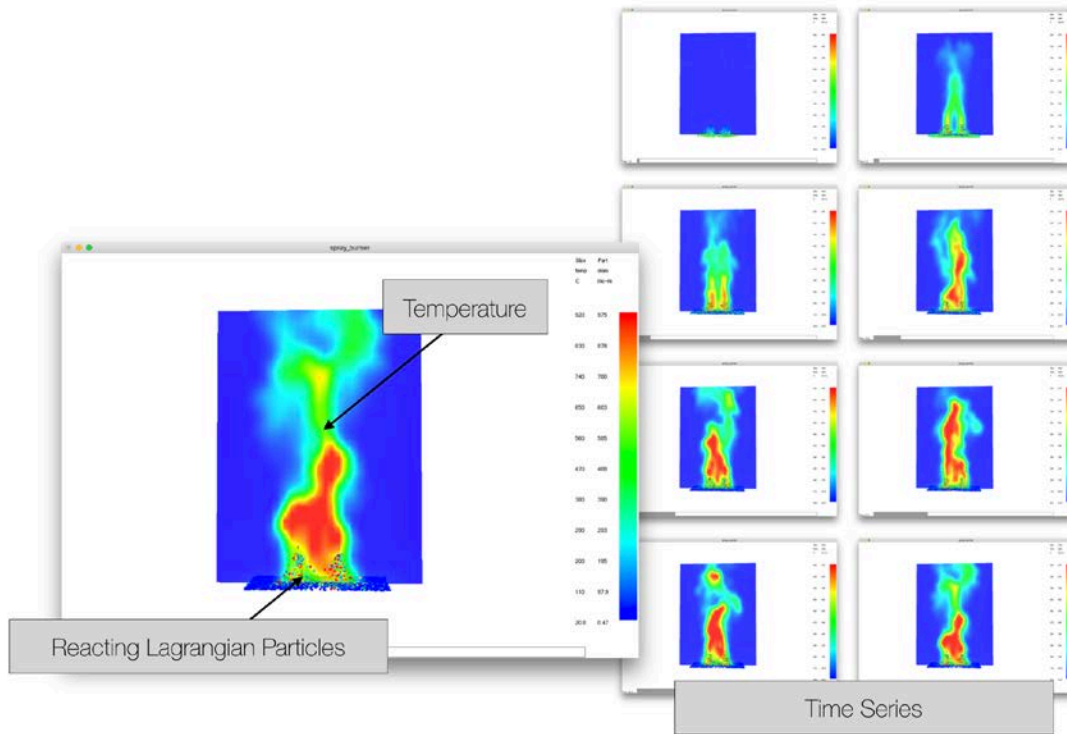
Figure 7: A standard FDS validation case which includes reacting Lagrangian particles interacting with an Eulerian flow field.
