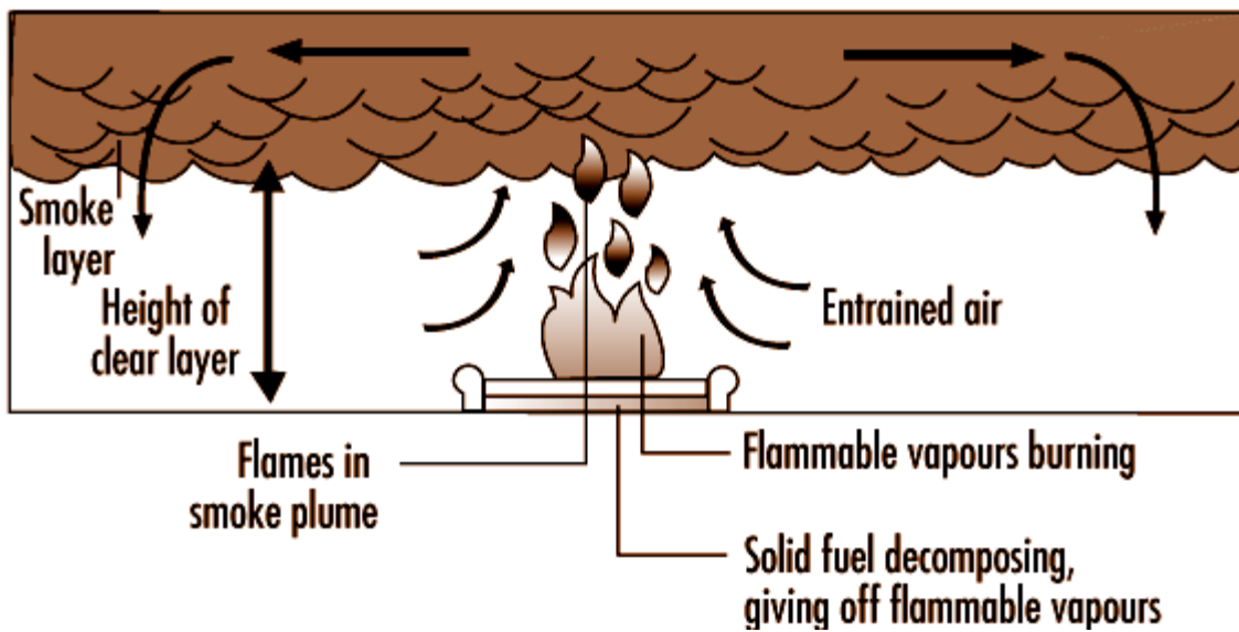
Figure 4: Smoke and hot gas layer formation and behavior.
