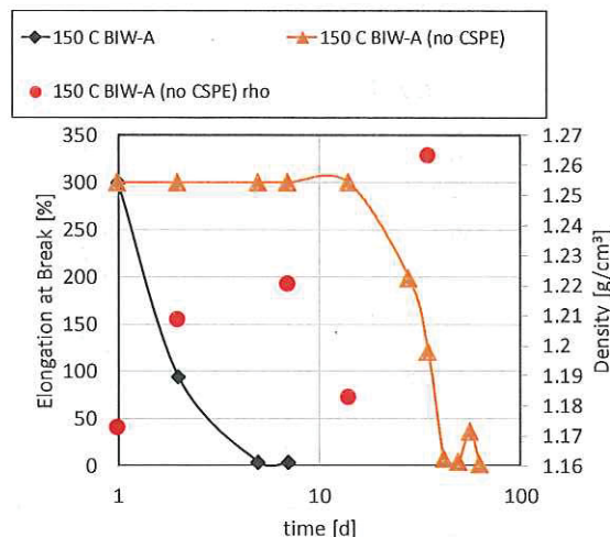
Fig. 16. EAB and density cable insulation data for BIW-A with and without the outer CSPE covering removed for the BIW-A.
