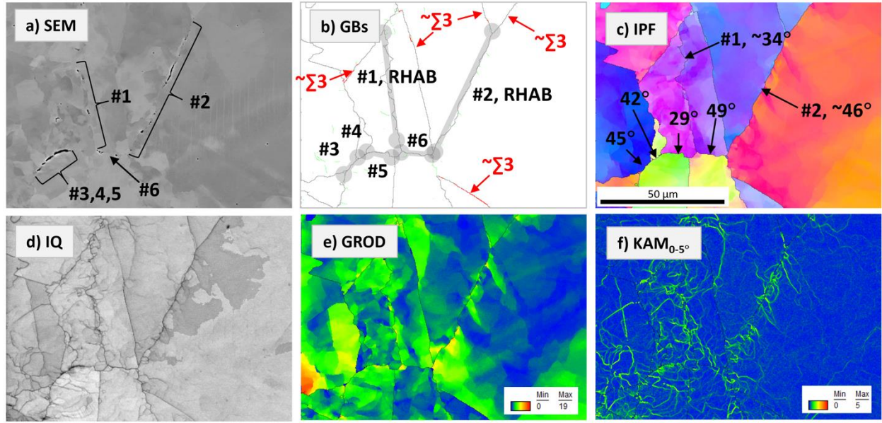
Figure 17. Helium-induced damage on GBs. (a) SEM/BSE image of the TMAZ ( \sim 0.15 mm from SZ boundary) with identified GB damage; (b) EBSD-retrieved GB network map; (c) IPF map, showing the misorientation of GBs #1-#6; (d, e, f) additional EBSD maps showing pattern quality (IQ map) and misorientation parameters. Scale bar is the same for all images. The SEM image was recorded at the 0^\circ tilt, whereas EBSD scans were performed at 70^\circ tilt. EBSD step (pitch) is 250 nm.
