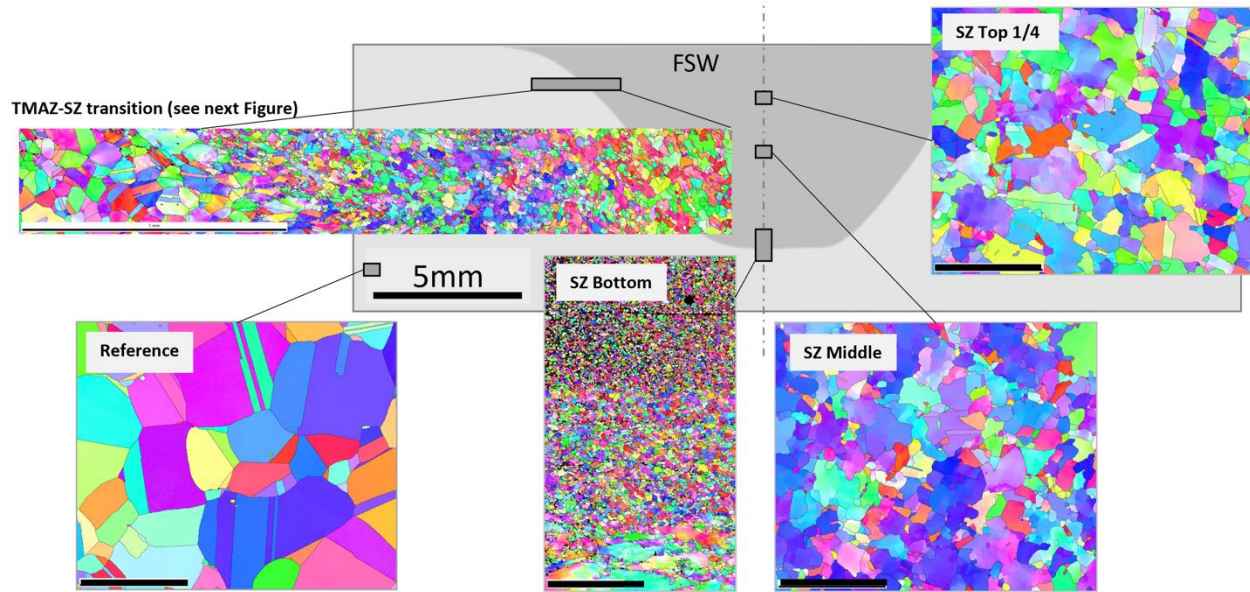
Figure 27. Microstructure of the friction stir weld with 15.6 appm He at key locations. The scale bar is the same for all IPF maps ( \approx 100 \mu\text{m} ), except the stitched TMAZ-SZ map (top left panel).
