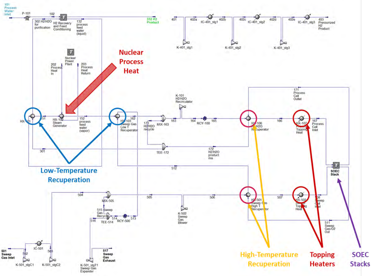
Figure B-4. Simplified HTE process flow diagram.
